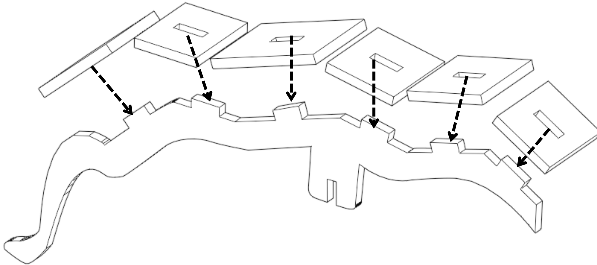
Assembled View:
