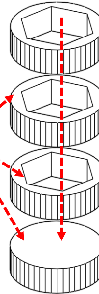
Socket Assembly
